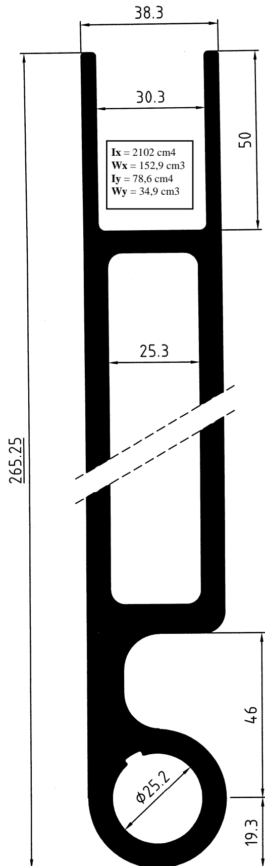
FT 61974 10,56 kg/m code 418917 7,50 m
