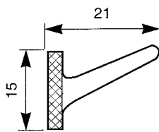
AN 8 AS 0,1 kg/m code 444020 100 m
